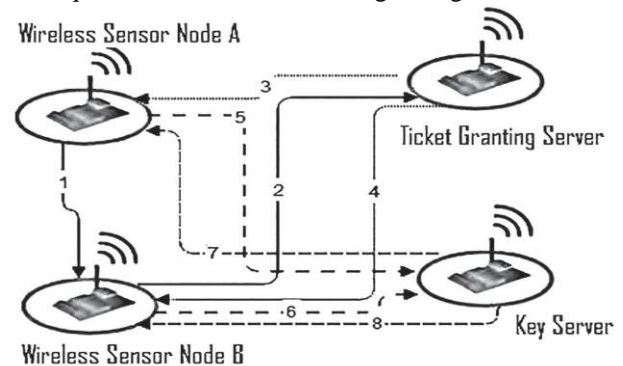
Figure 2. Illustration of the steps of the proposed node-to-node key agreement.
